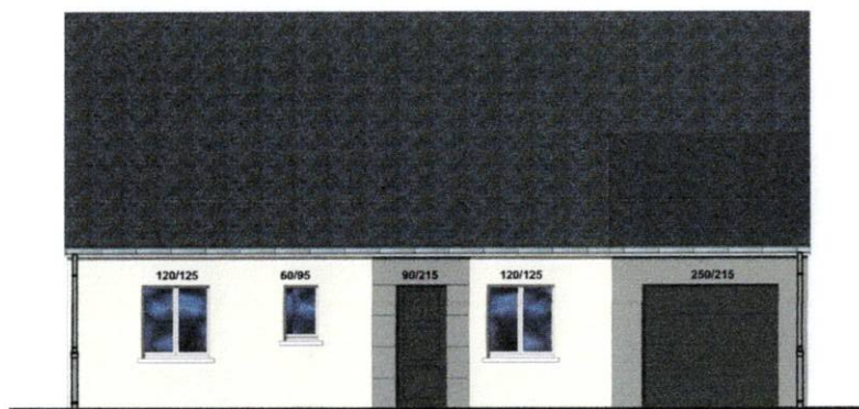
FACADE SUD
